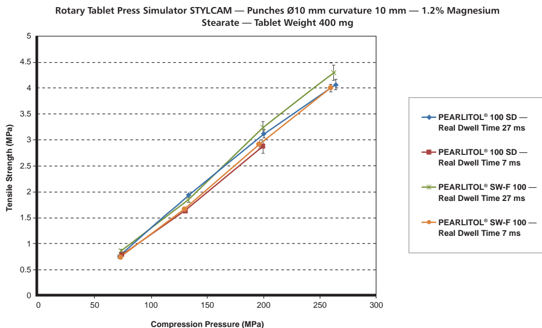
Figure 1: Tablet Simulator Results for PEARLITOL® SW-F 100 and PEARLITOL® 100 SD
