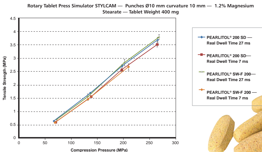
Figure 2: Tablet Simulator Results for PEARLITOL® SW-F 200 and PEARLITOL® 200 SD
