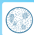
MICROALGAE
