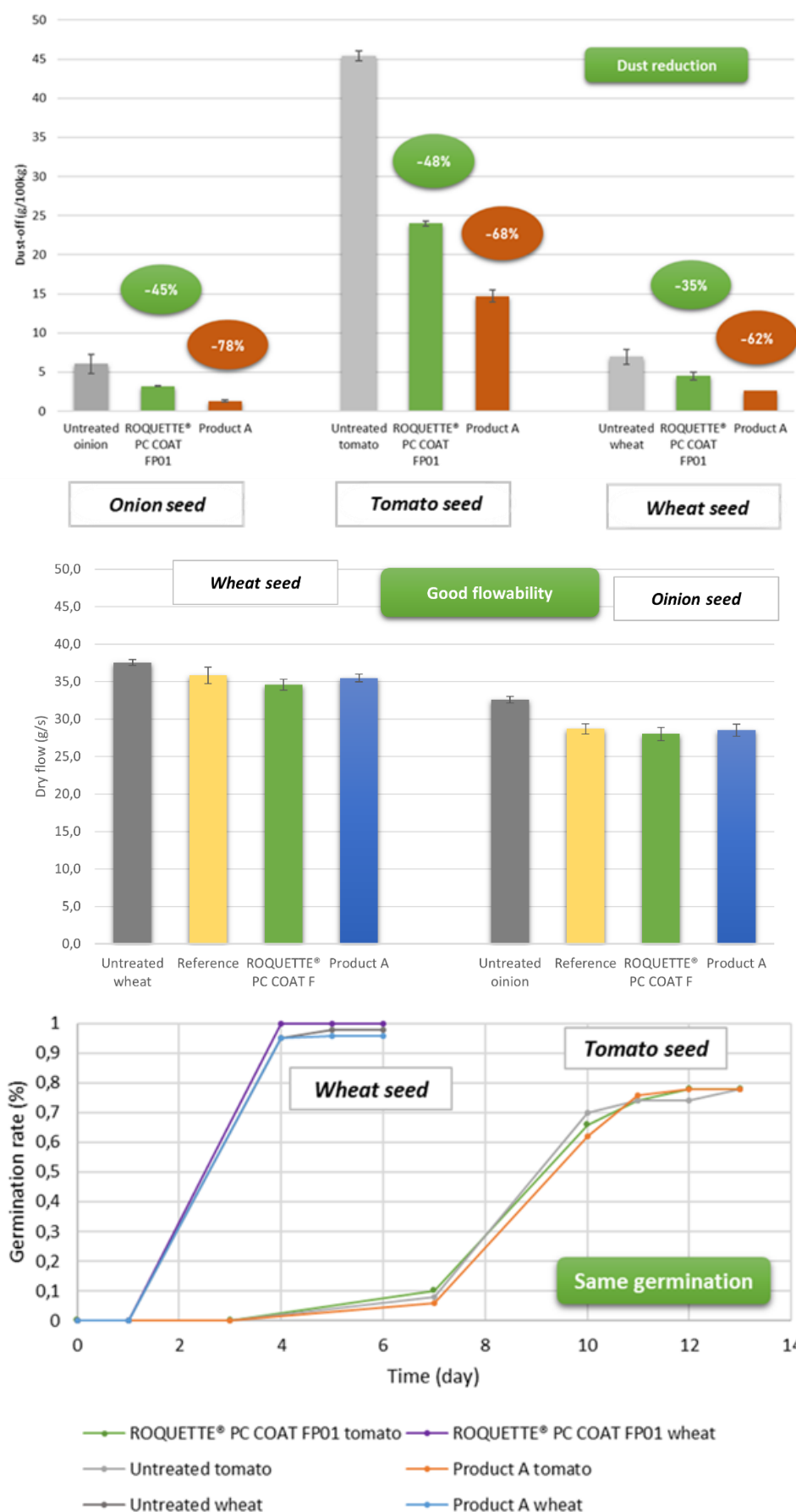
Figure 3: Dust reduction, flowability and germination data for seeds coated with ROQUETTE® PC COAT FP-01 and Product A solutions confirm their suitability for seed coating; performance is comparable to a commercial synthetic binder (where assessed).
