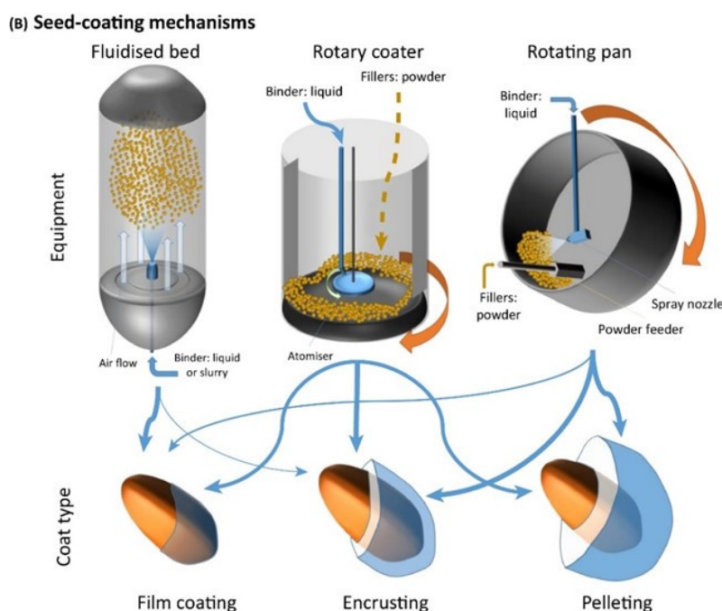
Figure 1: Examples of processes used for seed treatment and the resulting products 8
